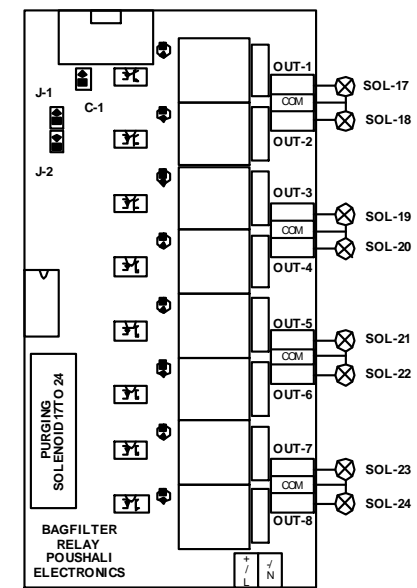
SAMPLE WIRING DIAGRAM FOR 4CHAMBER 8RELAY OFF LINE BAG FILTER TIMER POUHALI ELECTRONICS
