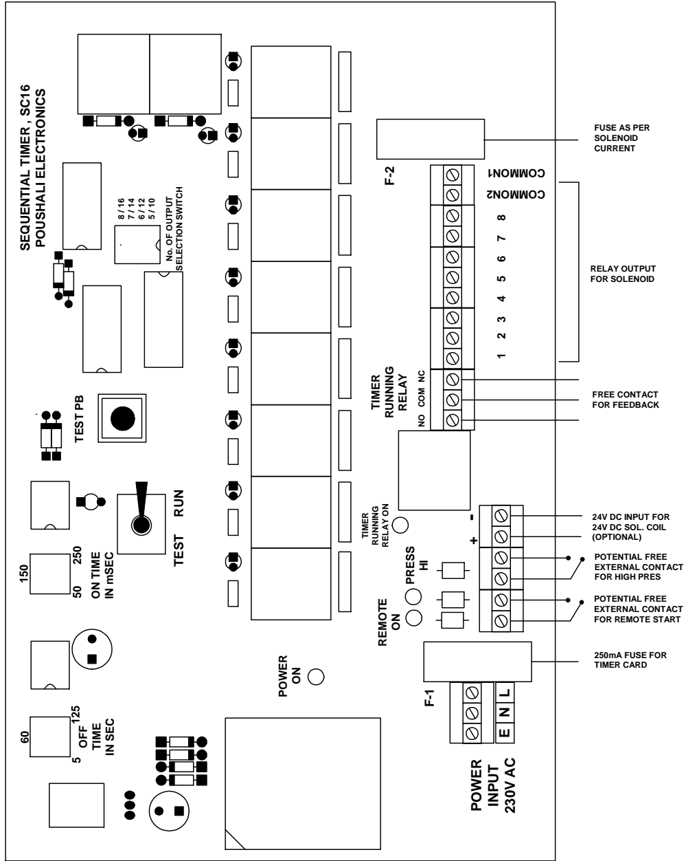
LAYOUT DIAGRAM OF BAG FILTER TIMER POUSHALI ELECTRONICS
